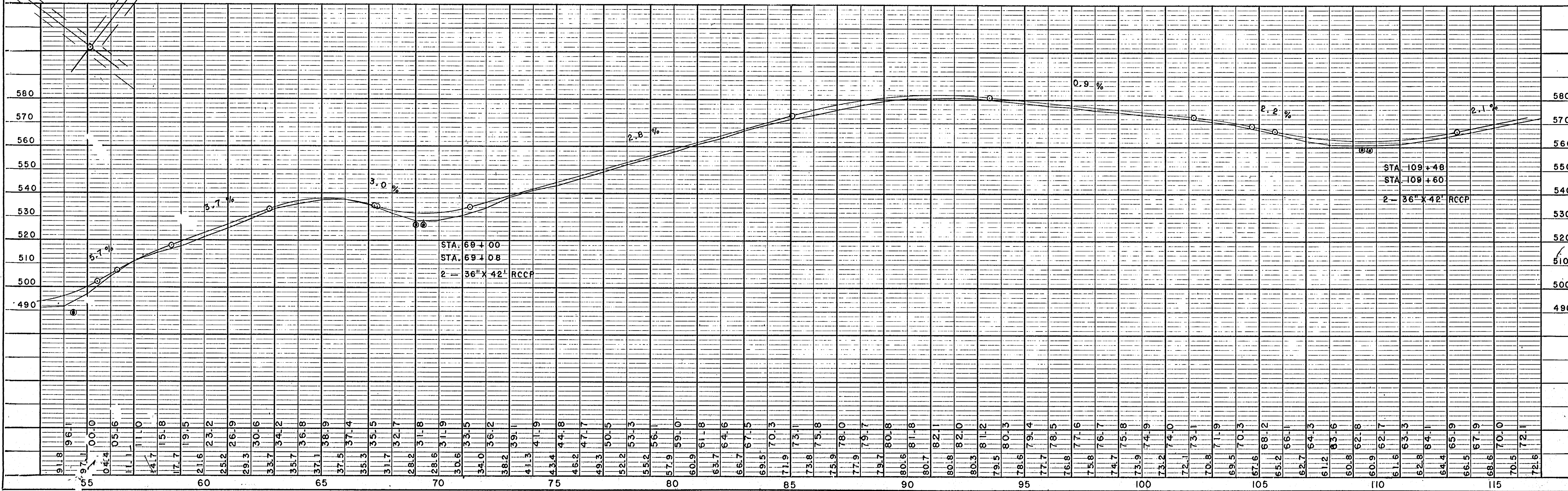
PLATE 1-PLAN-PROFILE O.P.R. & R.E. STANDARD THE HOLLISTON MILLS, INC. CHICAGO
