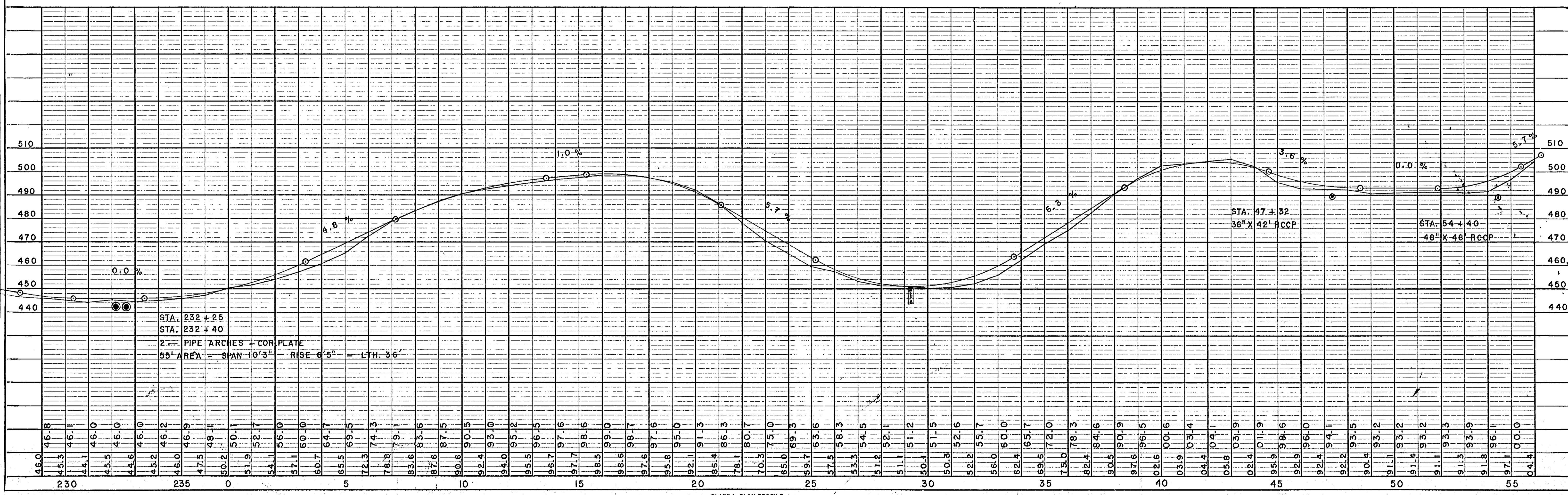
PLATE 1-PLAN-PROFILE © P.R.A.R.E. STANDARD THE HOLLISTON MILLS, INC. CHICAGO
